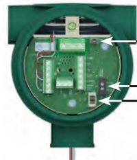
Separate USB Communication Channel 3-Way Switch for the 4-20 mA Output On/Off Power Switch
